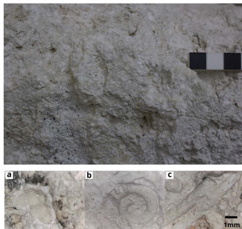
Figure 7. Macro-photo of carbonate rock of the cippus. Various fossils were observed in the carbonatic rock of the cippus: (a) gastropods; (b) ammonites; (c) algae tallus.
